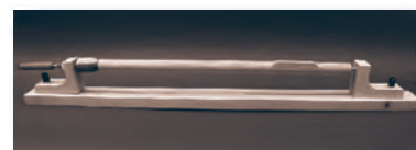
Flute Shaping and Sanding Jig
